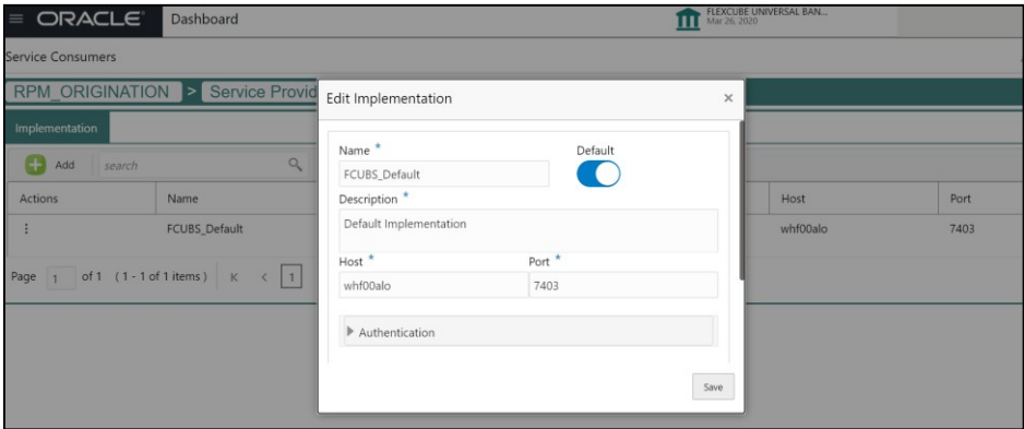
Figure 11: Edit Implementation
